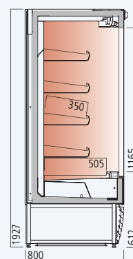
UNITED 80 AQP heated model
