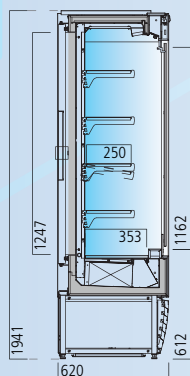
UNITED 62 PT chilled pass-through model
