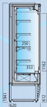
UNITED 62 chilled models
