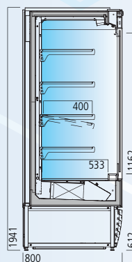
UNITED 80 chilled models
