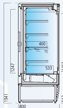
UNITED 80 PT chilled pass-through model
